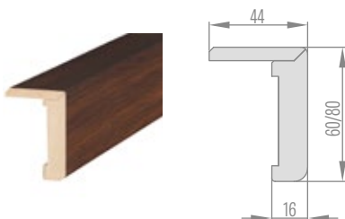
REGULAR SQUARE TO ADJUSTABLE FRAME
