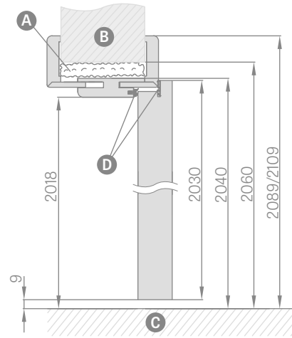
TECHNICAL PICTURE OF HERSE ADJUSTABLE FRAME
