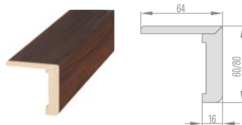
SQUARE WITH EXTENDED FEATHER TO ADJUSTABLE FRAME
