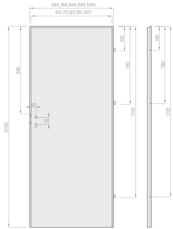
rebated door leaf
