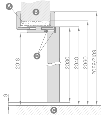
TECHNICAL PICTURE OF HERSE ADJUSTABLE FRAME
