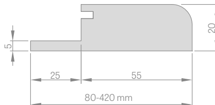
ADJUSTABLE WOODEN THRESHOLD
